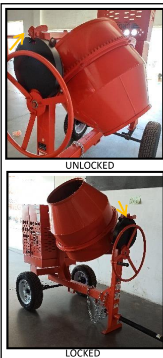
Fig. 5 BREAK LEVER AND LOCK ASSEMBLY
